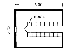
⑮ Plan of stall
